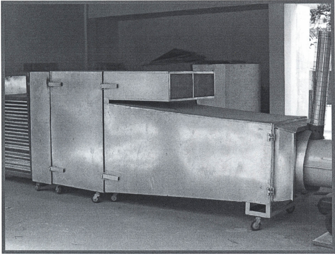
Fig. 1: The Developed Mobile Tunnel Dryer Used to Dry the Fruits
